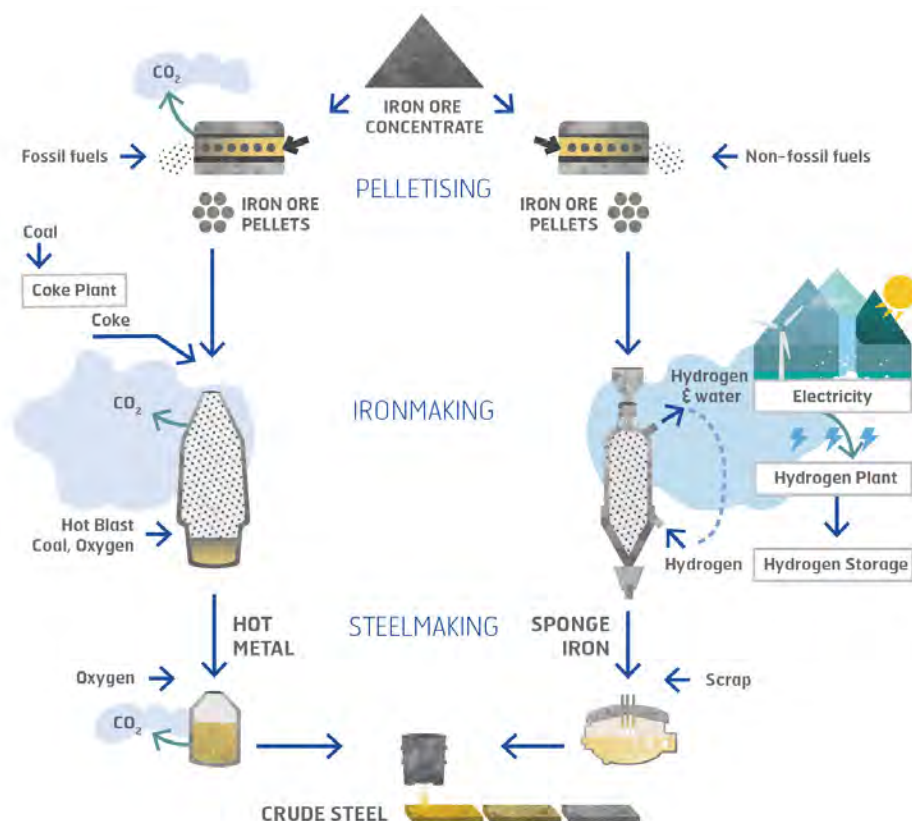
FIGURE 6.2 HYBRIT concept image
