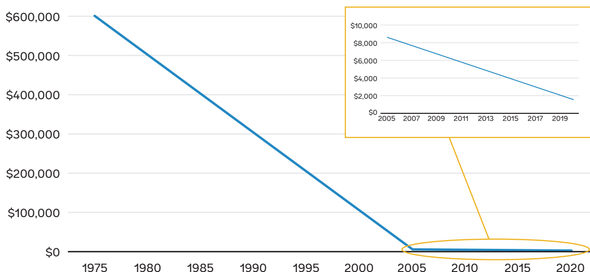
FIGURE 3.10 Stationary PEM fuel cell cost per kW
