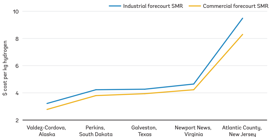
FIGURE 3.8 Spread in United States hydrogen prices from HyDRA, April 2019
